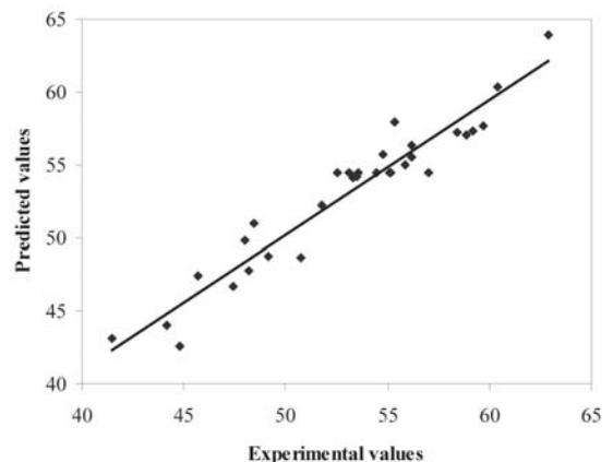
Figure 1. Experimental vs. predicted values plot of reducing sugars (g/L) from a liquefaction hydrolysis of SP by \alpha -amylase
